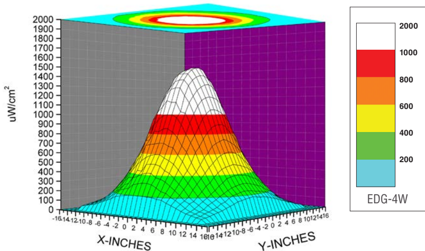
Surface Contour Profile for EDG-4W at 4 Feet (122cm)
