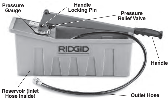
Figure 1 – 1450 Pressure Test Pump
