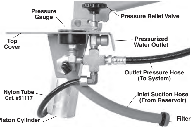
Figure 2 – Pump Components
