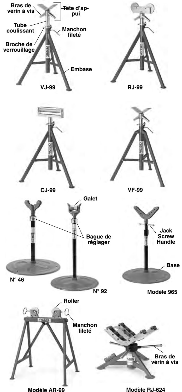
Figure 1 – Porte-tubes RIDGID
